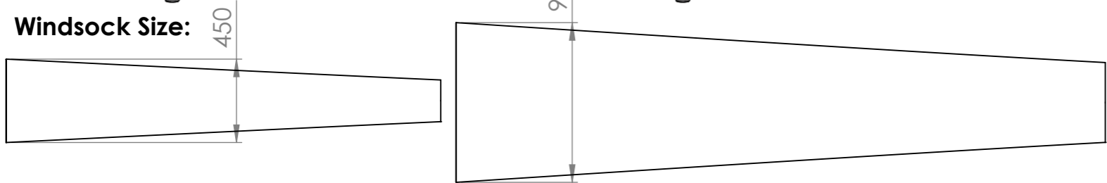
Windsock Size: 450 Size 1: Ø0.45 m x 2.50 m (Ø18" x 8 feet) Size 2: Ø0.9 m x 3.75 m (Ø36" x 12 feet)
