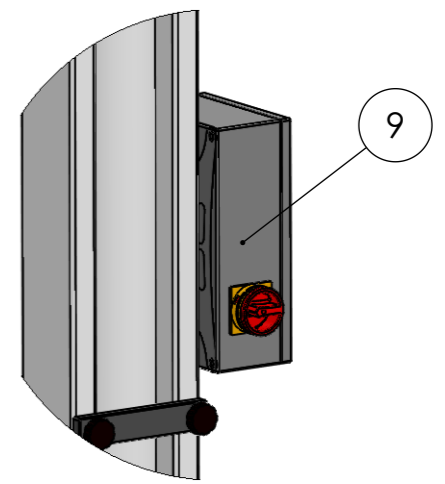
DETAIL D SCALE 1 : 10
